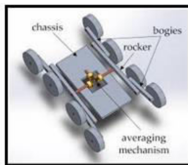
Fig 4: Rocker Frame
